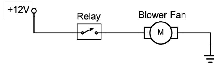
Figure 2 – A relay on the Opta PLC is used to automatically switch the blower fan ON and OFF.
